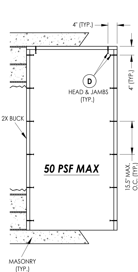
2X BUCK ANCHORING
